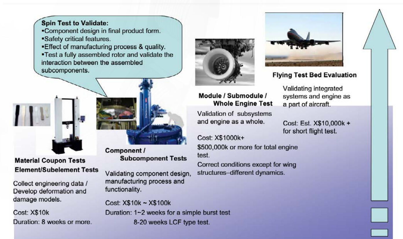
Figure-4 – Comparison of Spin Testing and Other Forms of Jet Engine Tests.
