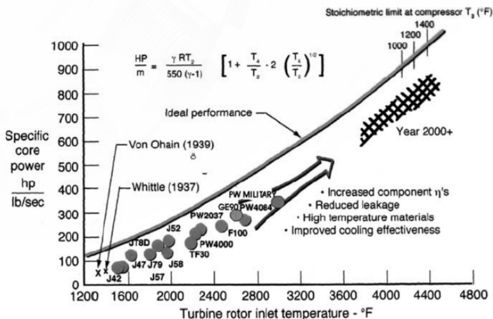
Figure-1 - Specific Core Power vs. Turbine Inlet Temperature (Courtesy of [3])
