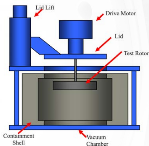
Figure-2 – Spin Test Rig
