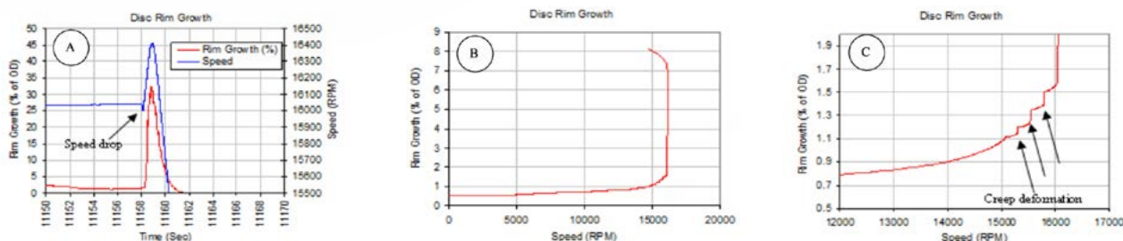
Figure-13 – Disc growth behavior towards a disc burst. A) Speed and disc rim growth at the instance of disc burst. B) Speed vs. Disc Rim Growth, C) Zoomed view of the growth curve near the knee.
