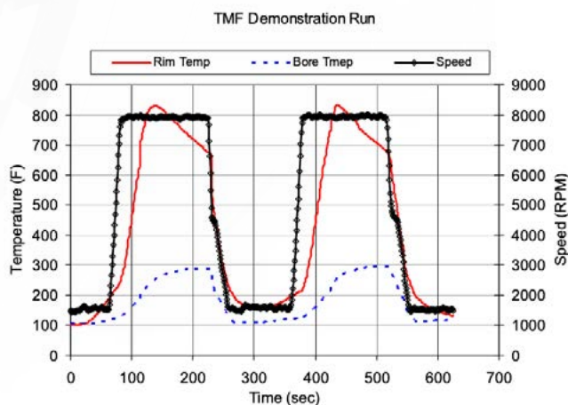
Figure-12 – TMF Rig Demonstration.
