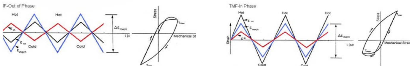
Figure-10 – TMF Cycles (Courtesy of [15]).
