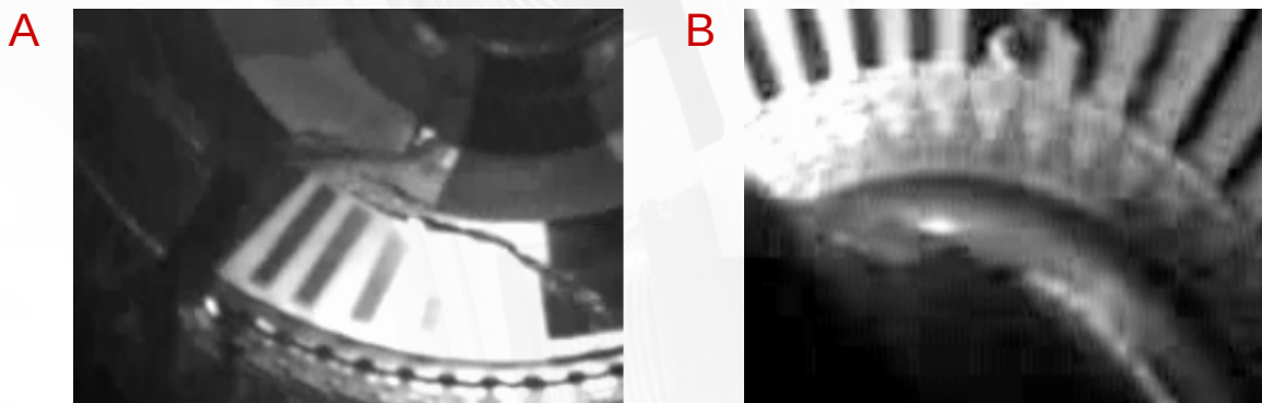
Figure-15 – High speed video images of a disc burst (a) and blade liberation at elevated temperature (b).
