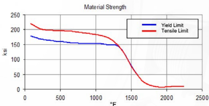
Figure-5 – Temperature Dependent Behavior of IN718 Alloy.
